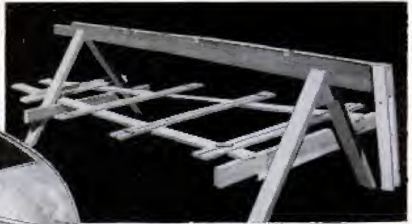
Boat is assembled upside down with a mold board being used in some cases. Mold board is raised on horses, above, so tops of boat frames clear floor
